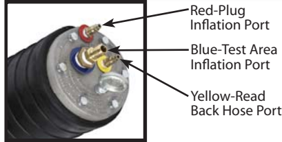
Front Plug
