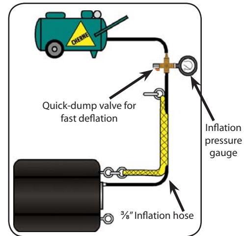
Poly-lift line with gauge
